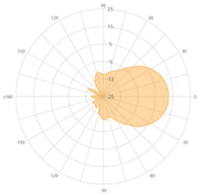
N5-X12 (12 dBi)
