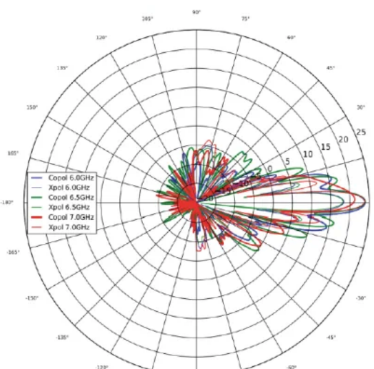
Elevation, Vertical
