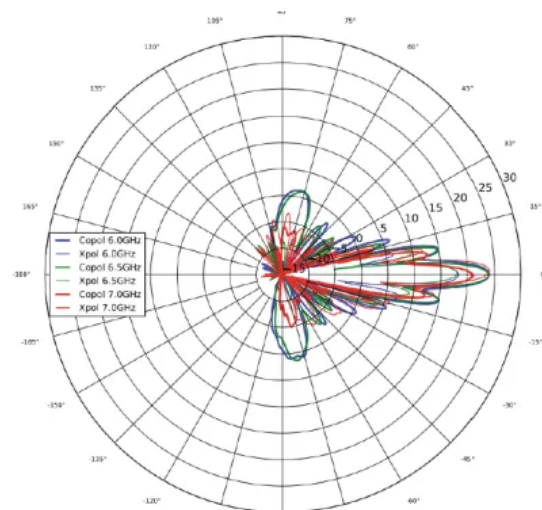
Azimuth, Vertical
