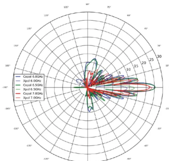
Elevation, Horizontal
