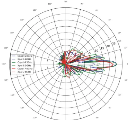
Azimuth, Horizontal
