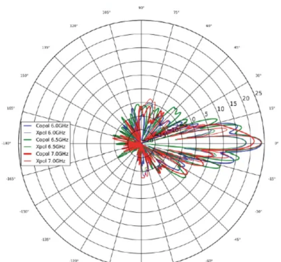
Elevation, Vertical
