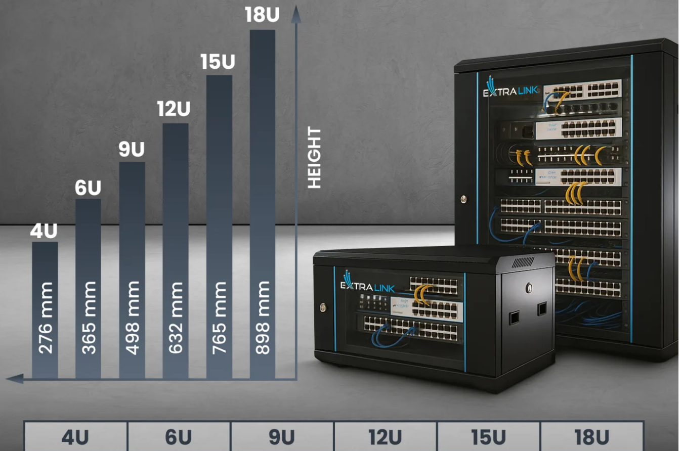
Extralink 9U 600x450 Black | rack | wall-mounted cabinet
