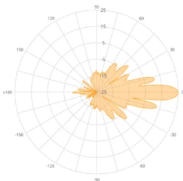
N5-X25 (25 dBi)
