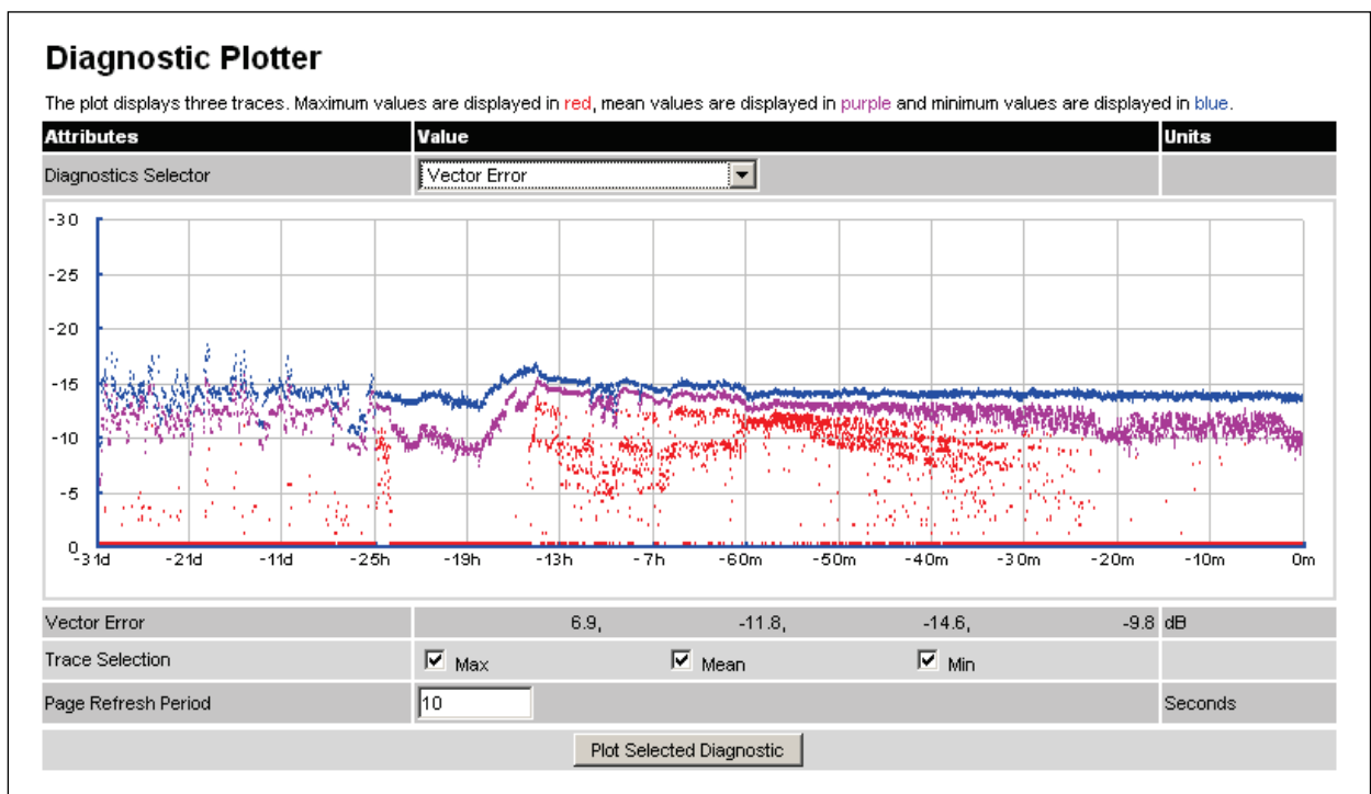
Figure 238 Diagnostic Plotter page (PTP topology)
