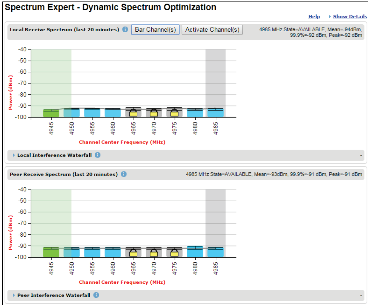
Figure 213 Barred channels
