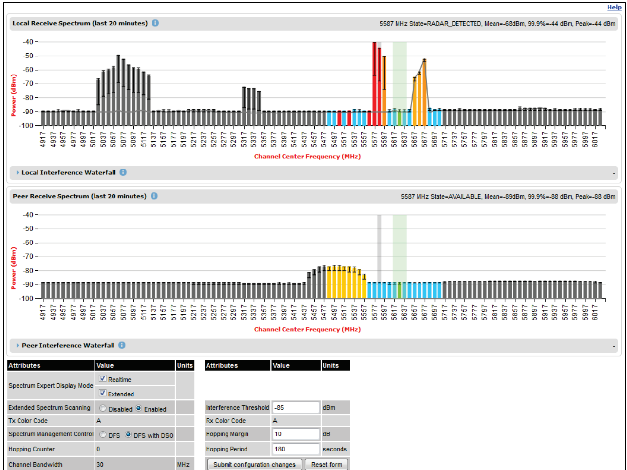
Figure 210 Spectrum Expert page with radar avoidance - Extended Display
