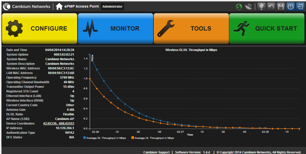
Figure 13 GUI dashboard
