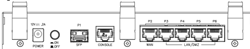
Figure 51 ATP100W Rear Panel
