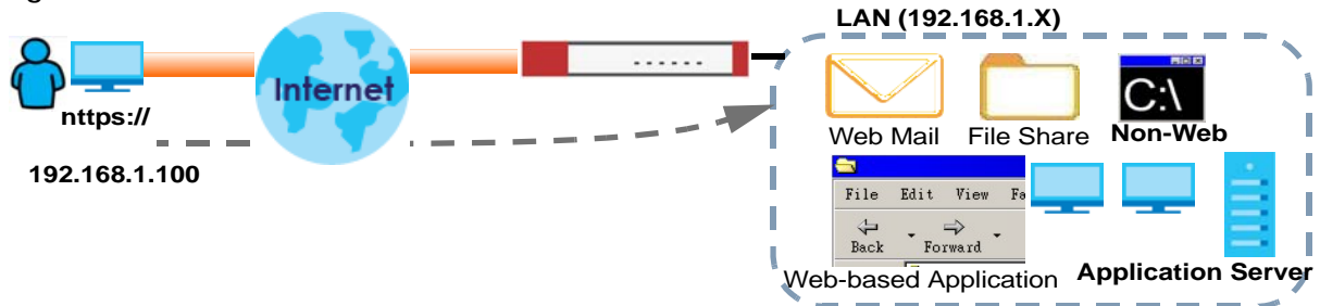
Figure 327 Network Access Mode: Full Tunnel Mode
