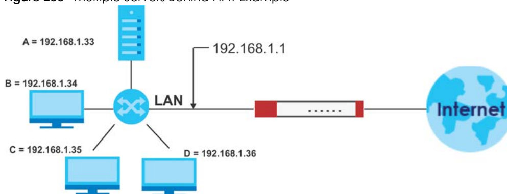
Figure 256 Multiple Servers Behind NAT Example
