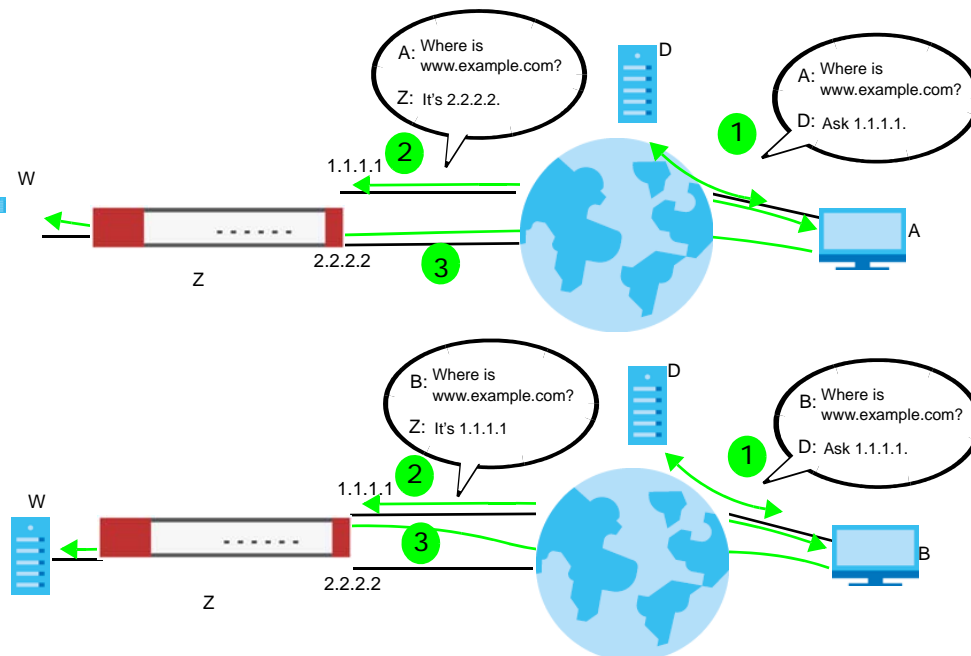
Figure 304 DNS Load Balancing Example
