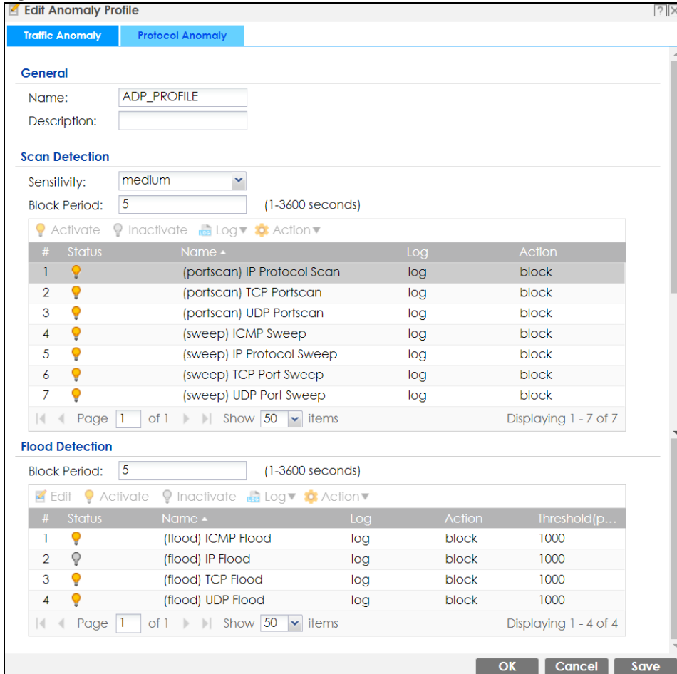
Figure 374 Configuration > Security Policy > ADP > Profile > Add-Traffic-Anomaly
