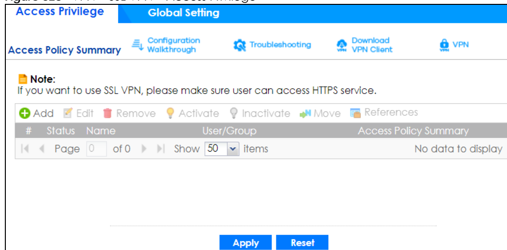
Figure 328 VPN > SSL VPN > Access Privilege
