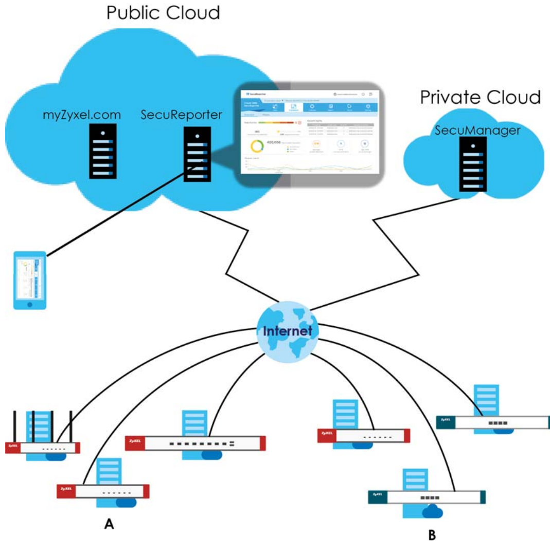
Figure 554 Cloud CNM SecuReporter Application Scenario
