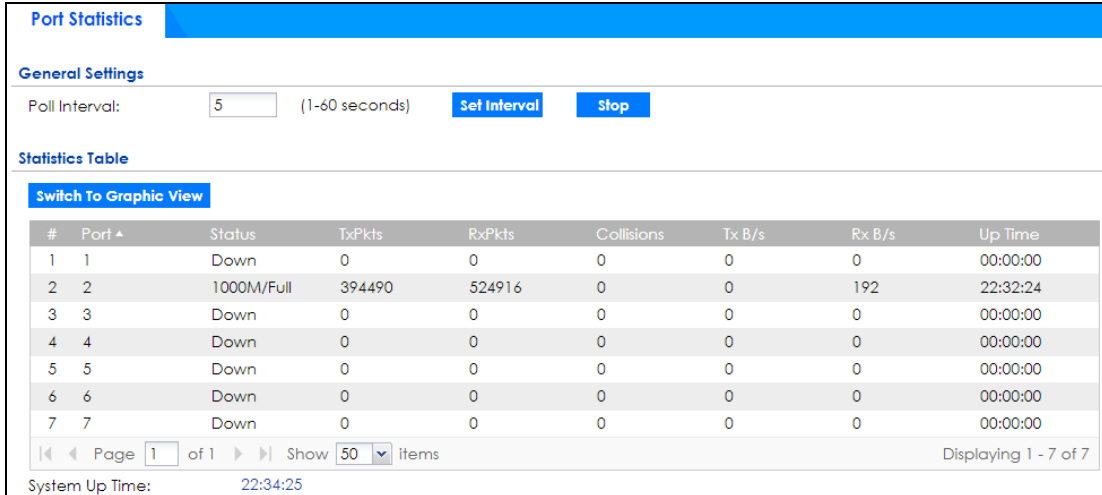
Figure 118 Monitor > System Status > Port Statistics
