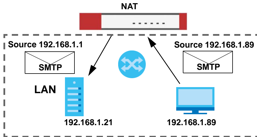
Figure 260 LAN to LAN Traffic
