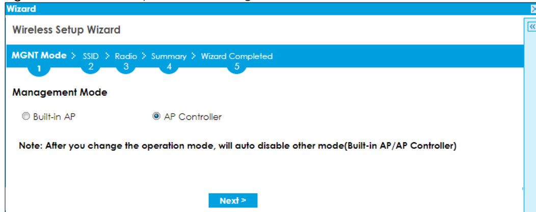
Figure 98 Wireless Setup Wizard > Management Mode
