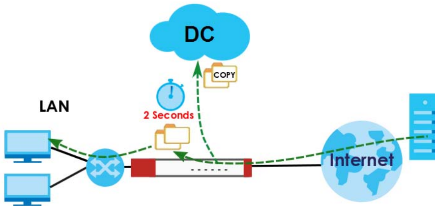
Figure 443 Advanced Zyxel Sandbox Inspection
