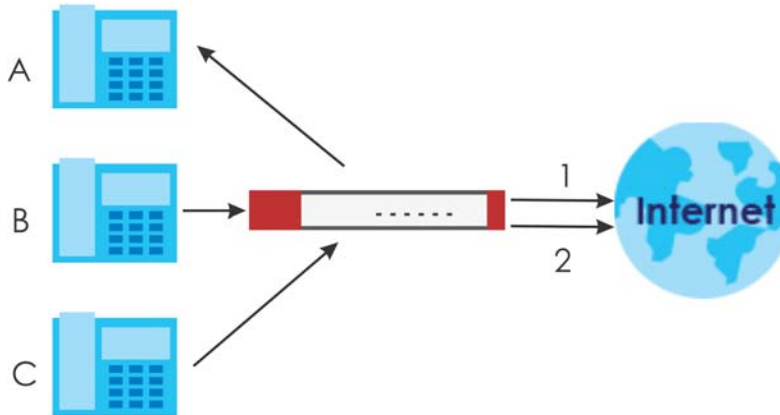
Figure 273 VoIP Calls from the WAN with Multiple Outgoing Calls
