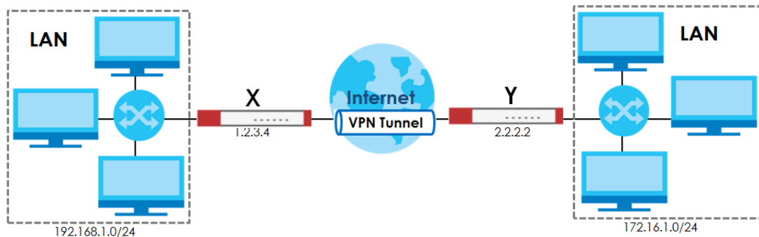
Figure 326 Site-to-site IPsec VPN Example
