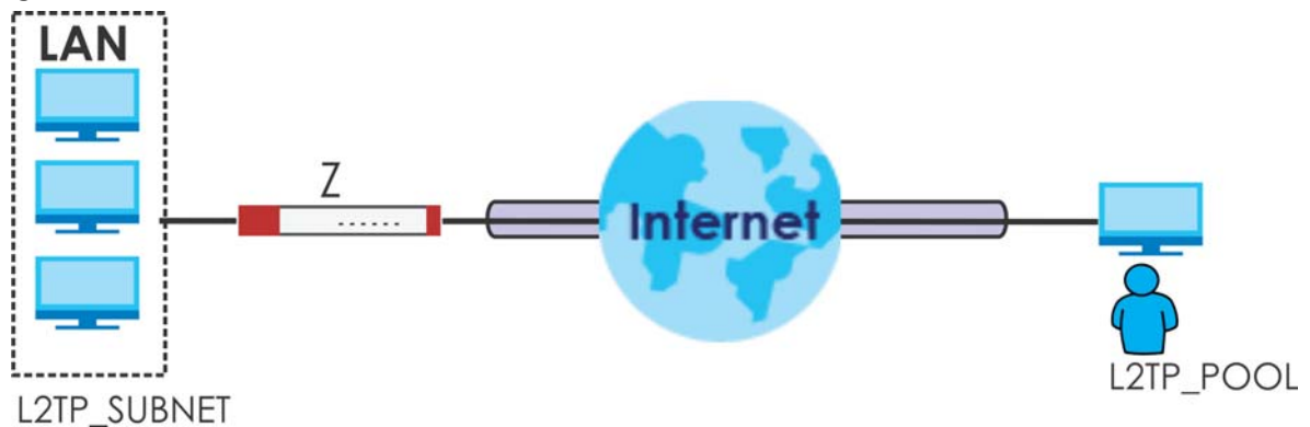
Figure 332 Policy Route for L2TP VPN
