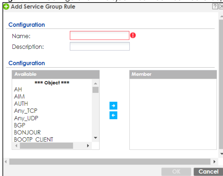
Figure 511 Configuration &gt; Object &gt; Service &gt; Service Group &gt; Edit
