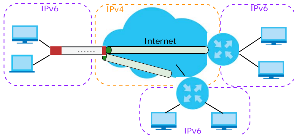
Figure 215 6to4 Tunnel
