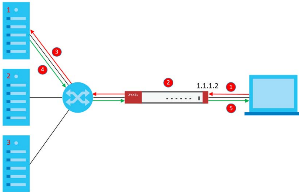
Figure 264 Load Balancing Process
