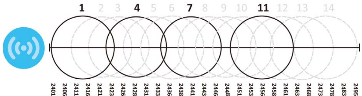
Figure 192 An Example Four-Channel Deployment
