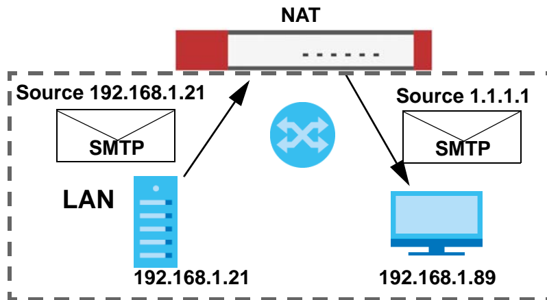
Figure 261 LAN to LAN Return Traffic
