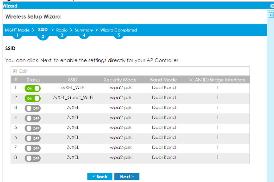
Figure 99 Wireless Setup Wizard > SSID - AP Controller
