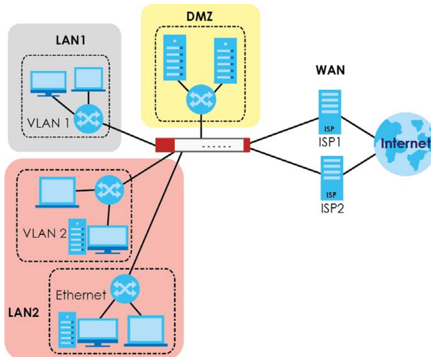
Figure 466 Example: Zones
