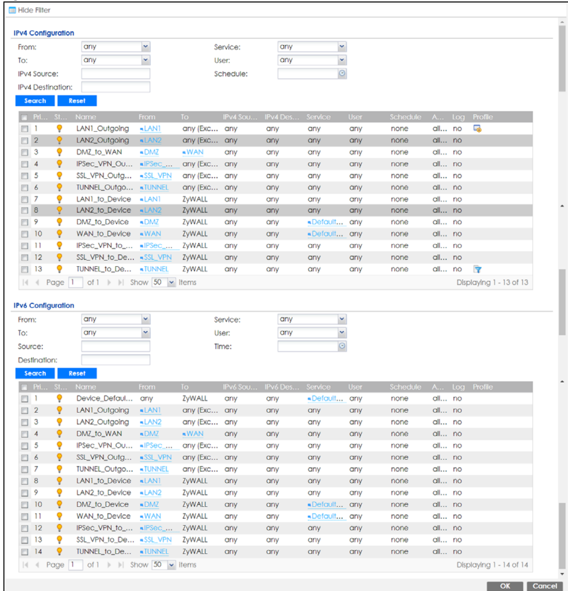
Figure 385 Configuration > Security Service > Content Filter > Action
