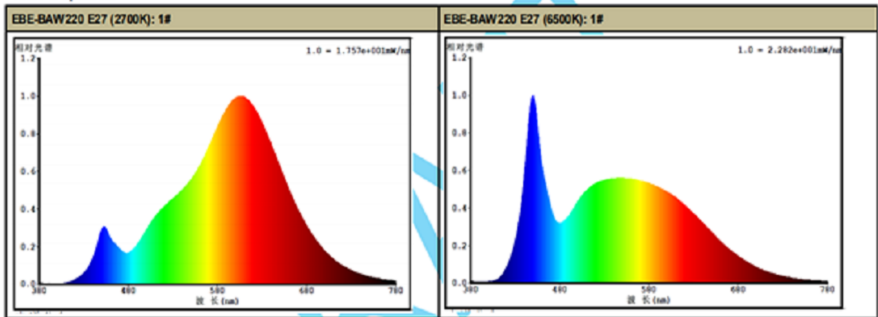
Figure 6: Spectrum
