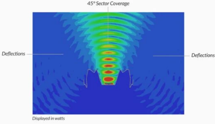
Near Field of AM-5AC22-45
