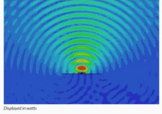
Near Field of Standard Sector Antenna
